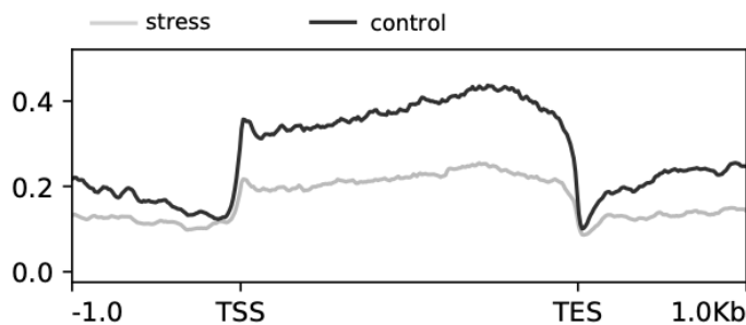
Figure 5: Combined metagene ATAC profiles of stressed and control daphnia populations. X-axis in base-pairs. TSS = Transcription start site, TES = transcription end site. Y-axis average enrichment of ATAC-seq reads over genes and upstream and downstream regions.
